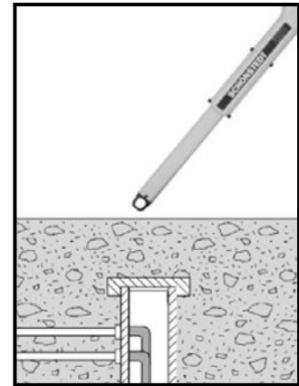
Figure 17. Locating Water Well Casings
