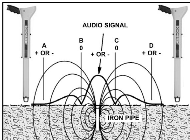
Figure 14. Signal Pattern from a Strongly Magnetized Marker
