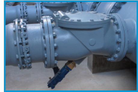
Swing-Flex® Check Valve with Oil Cushion for Pump Discharge
